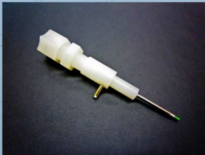
Overlook OneShot™ co-ax filler needle w/ Jaco connector and Teflon coating
